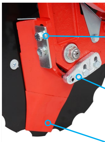
Shoe height adjustment screws
